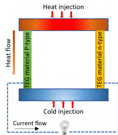
Figure 11. Schematic view of the thermoelectric materials and electric voltage producing process [17,84] (this drawing was created by the authors).
