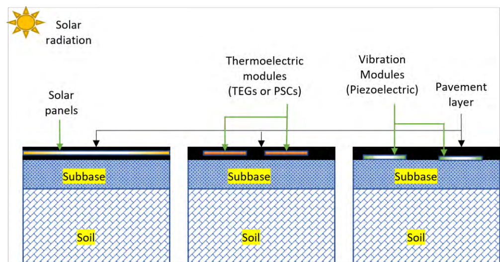
Figure 1. Schematic diagram illustrating pavement energy harvesting technologies [17]. (This drawing was created by the authors).
