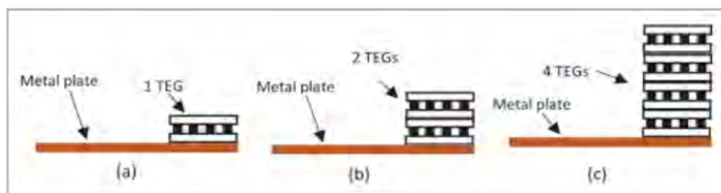
Figure 13. TEG module configurations; (a) 4 \times 1 , (b) 2 \times 2 , (c) 1 \times 4 [92].
