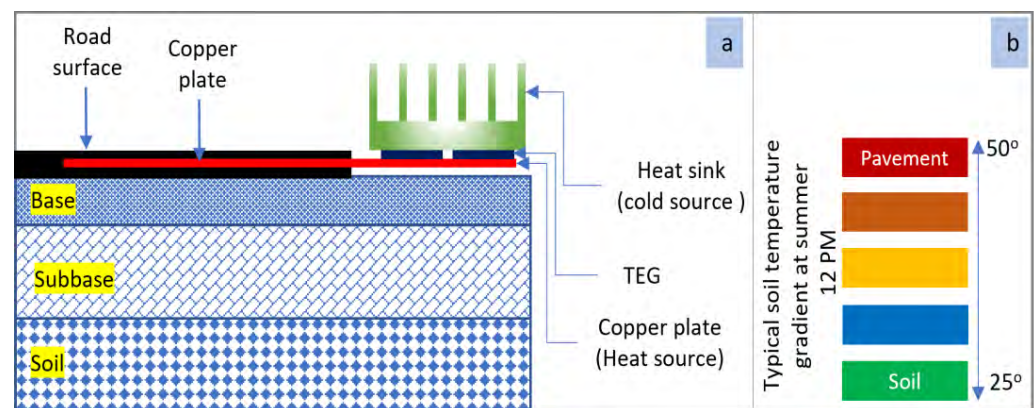
Figure 12. (a) Typical thermoelectric energy harvesting system in pavement [86,87] (b) temperature distribution in asphalt pavement [88,89] (this drawing was created by the authors).
