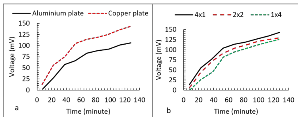
Figure 14. Output voltage vs. time (a) different materials, (b) different configurations [92].
