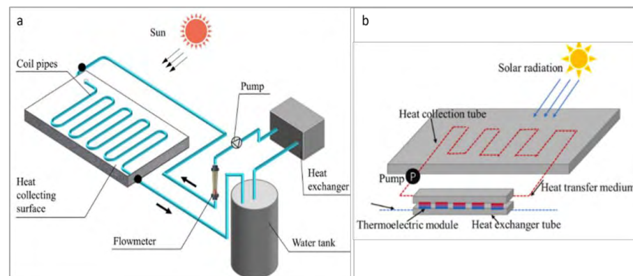
Figure 10. This 3D view illustrates the path solar collector system connected to (a) heat exchanger and (b) TEG modules [32,79,80].
